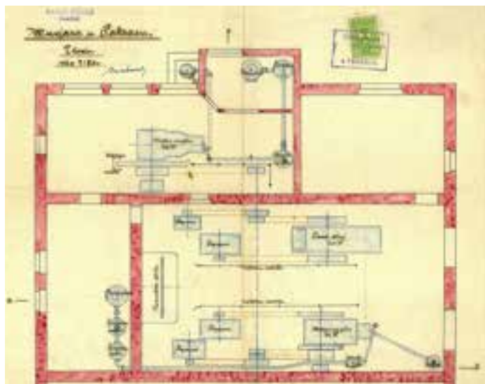
Munjara, Pakrac, tlocrt, Maurice Scheuer
