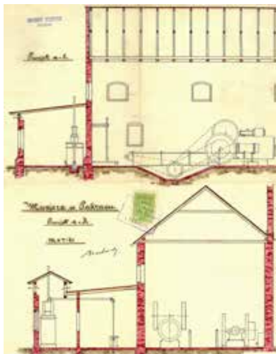
Munjara, Pakrac, nacrt, Maurice Scheuer
